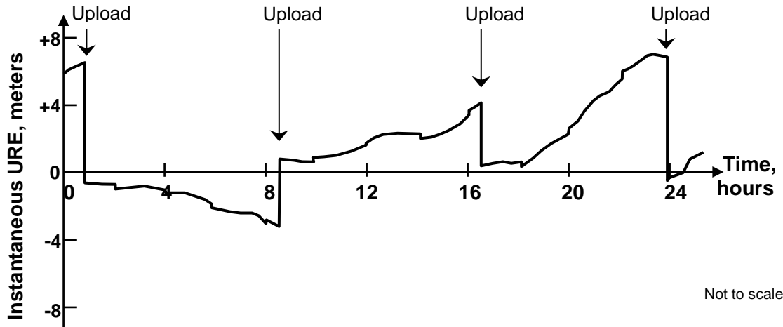
Figure A.4-5a. Instantaneous SPS SIS URE as a Function of Time
